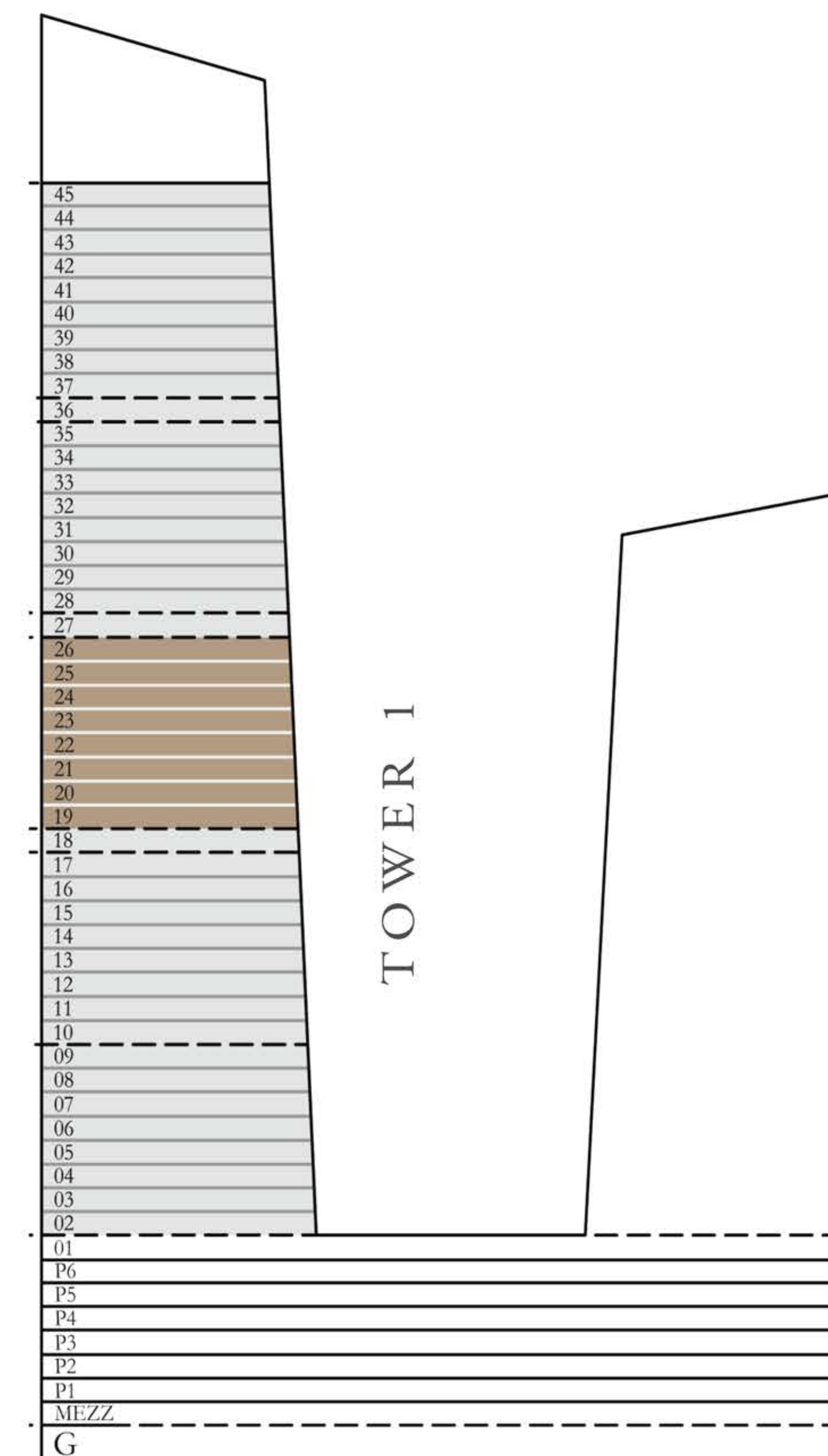
KEY SECTION-T1
