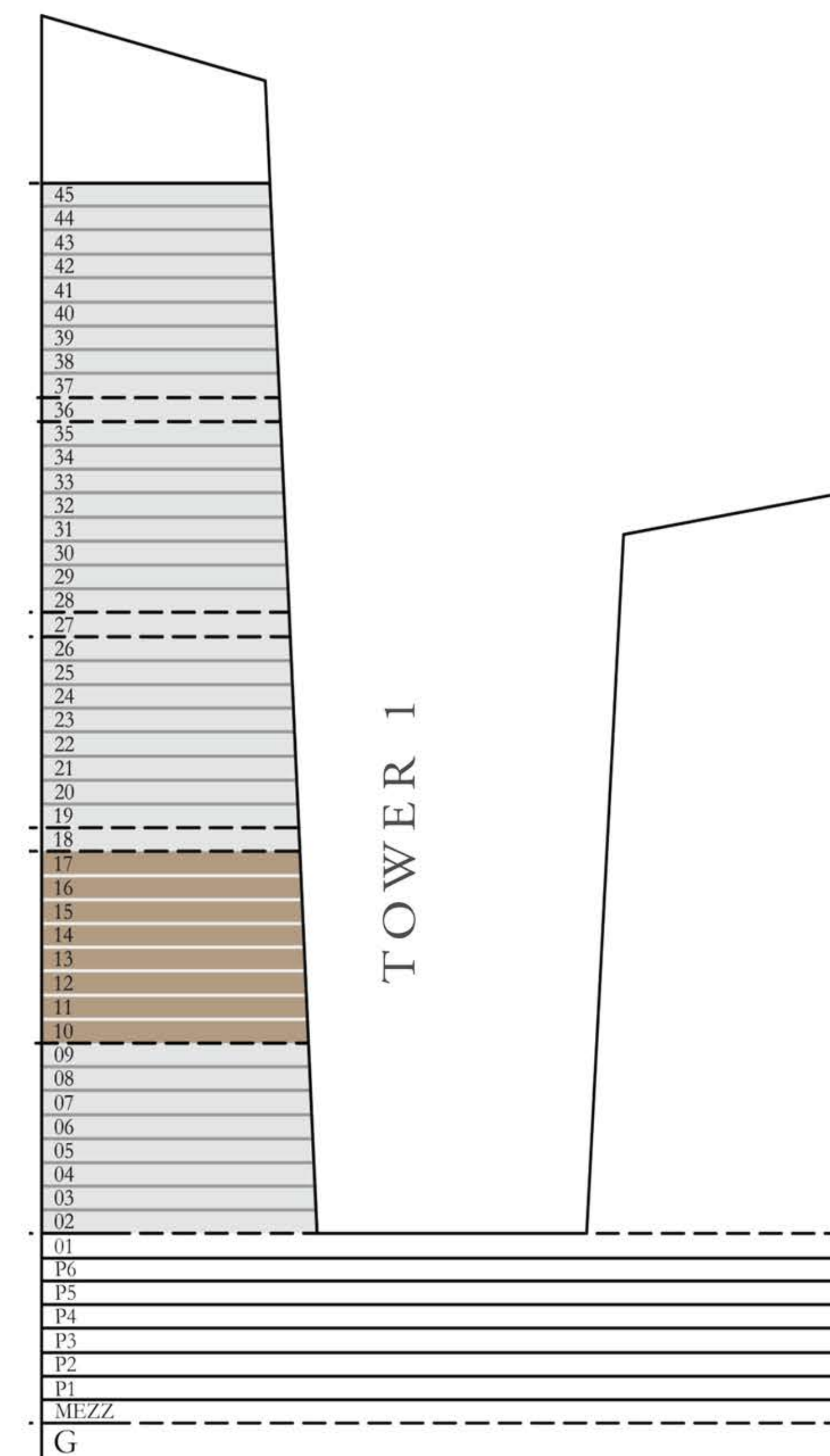
KEY SECTION-T1
