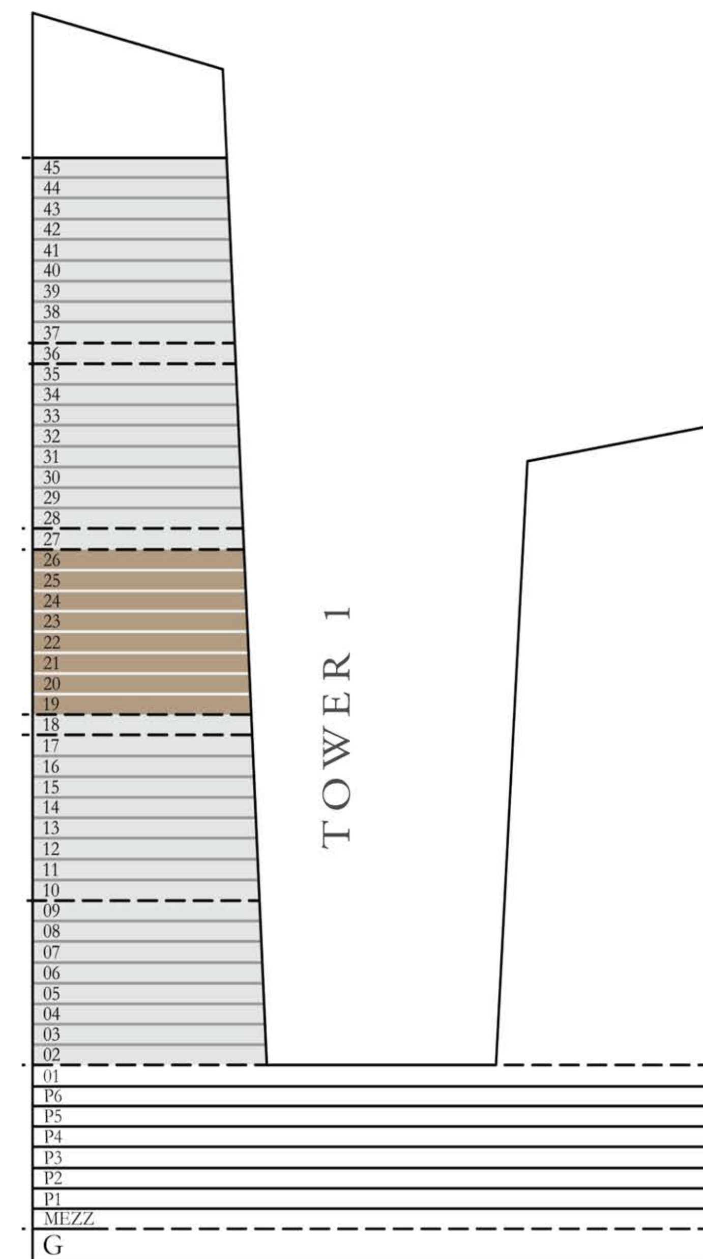
KEY SECTION-T1
